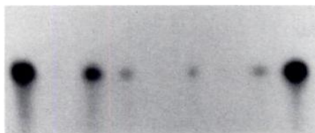
Fig. 4. Tissue distribution of the cloned meleagrid P 2Y purinergic receptor. RNase protection assays were performed on 25 µg of total RNA isolated from various meleagrid tissues, using a 274-base pair antisense ribonucleotide probe specific for the cloned meleagrid P 2Y purinergic receptor, as described in Experimental Procedures. B, brain; H, heart; Lu, lung; St, stomach; L, liver; GI, gastrointestinal tract; K, kidney; SM, skeletal muscle; Bl, blood.
