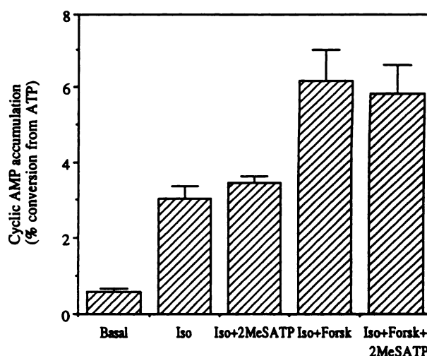
Fig. 3. Absence of 2MeSATP-promoted inhibition of cAMP accumulation in P_{2Y} receptor-transfected 1321N1 cells. 1321N1- P_{2Y} cells were pre-labeled with [ ^3H ]adenine overnight and subjected to a 30-min incubation in [ ^3H ]adenine-free medium, as described in Experimental Procedures. The labeled and washed cells were then incubated for 5 min in the absence of added drug (Basal) or in the presence of 10 \mu M isoproterenol (Iso), 10 \mu M isoproterenol plus 10 \mu M 2MeSATP (Iso+2MeSATP), 10 \mu M isoproterenol plus 10 \mu M forskolin (Iso+Forsk), or 10 \mu M isoproterenol plus 10 \mu M forskolin plus 10 \mu M 2MeSATP (Iso+Forsk+2MeSATP) and were assayed for cAMP accumulation as described in Experimental Procedures. The data shown are mean \pm standard error for three to nine experiments assayed in quadruplicate.
